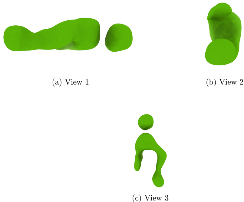
Figure 4: Isosurface at threshold=0.700000. Views generated by ChimeraX at a the following X, Y, Z angles: View 1 (0, -90, -90), View 2 (-90, 0, -90), View 3 (0, 0, 0).
