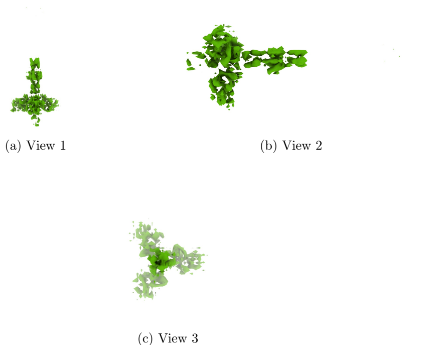
Figure 4: Isosurface at threshold=0.600000. Views generated by ChimeraX at a the following X, Y, Z angles: View 1 (0, -90, -90), View 2 (-90, 0, -90), View 3 (0, 0, 0).
