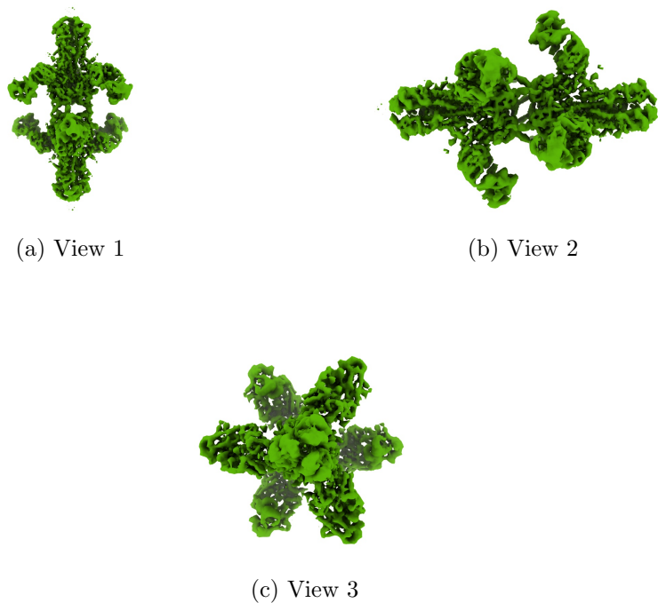
Figure 4: Isosurface at threshold=0.448000. Views generated by ChimeraX at a the following X, Y, Z angles: View 1 (0, -90, -90), View 2 (-90, 0, -90), View 3 (0, 0, 0).
