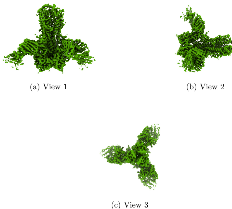
Figure 4: Isosurface at threshold=0.022400. Views generated by ChimeraX at a the following X, Y, Z angles: View 1 (0, -90, -90), View 2 (-90, 0, -90), View 3 (0, 0, 0).
