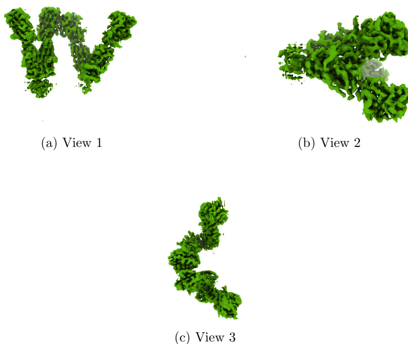
Figure 4: Isosurface at threshold=0.008500. Views generated by ChimeraX at a the following X, Y, Z angles: View 1 (0, -90, -90), View 2 (-90, 0, -90), View 3 (0, 0, 0).
