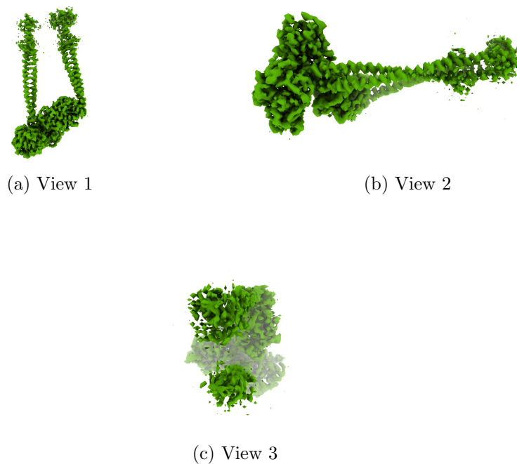
Figure 4: Isosurface at threshold=0.009900. Views generated by ChimeraX at a the following X, Y, Z angles: View 1 (0, -90, -90), View 2 (-90, 0, -90), View 3 (0, 0, 0).
