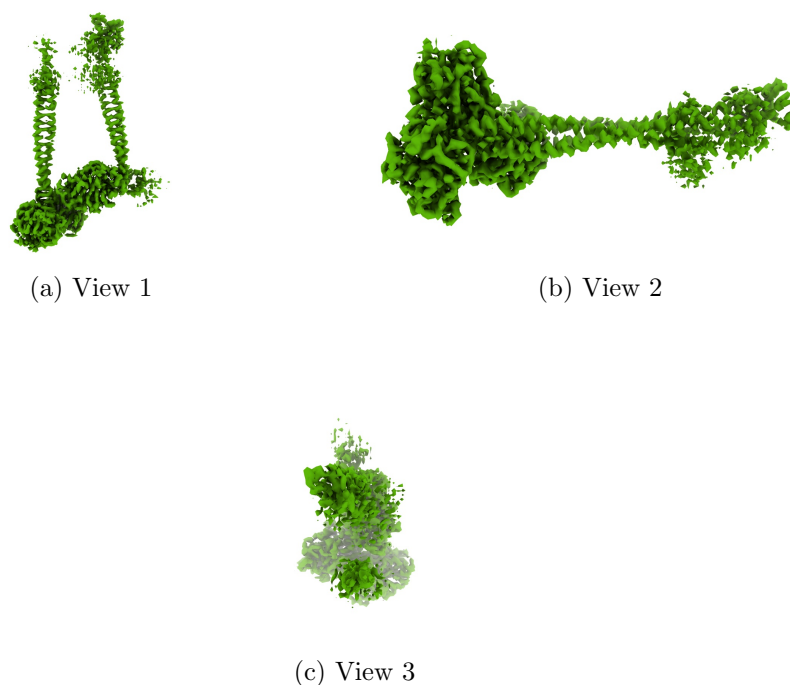
Figure 4: Isosurface at threshold=0.009920. Views generated by ChimeraX at a the following X, Y, Z angles: View 1 (0, -90, -90), View 2 (-90, 0, -90), View 3 (0, 0, 0).
