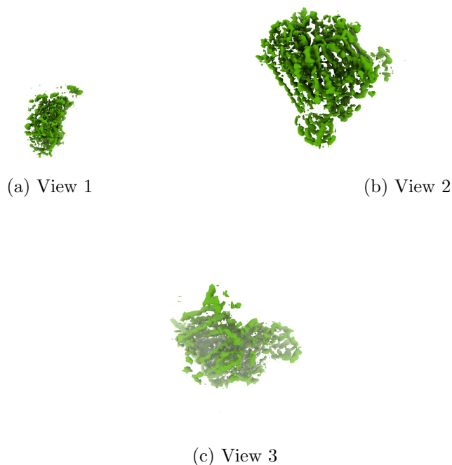
Figure 4: Isosurface at threshold=0.700000. Views generated by ChimeraX at a the following X, Y, Z angles: View 1 (0, -90, -90), View 2 (-90, 0, -90), View 3 (0, 0, 0).
