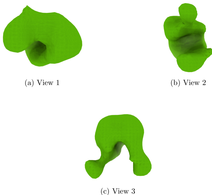
Figure 4: Isosurface at threshold=1.000000. Views generated by ChimeraX at the following X, Y, Z angles: View 1 (0, -90, -90), View 2 (-90, 0, -90), View 3 (0, 0, 0).
