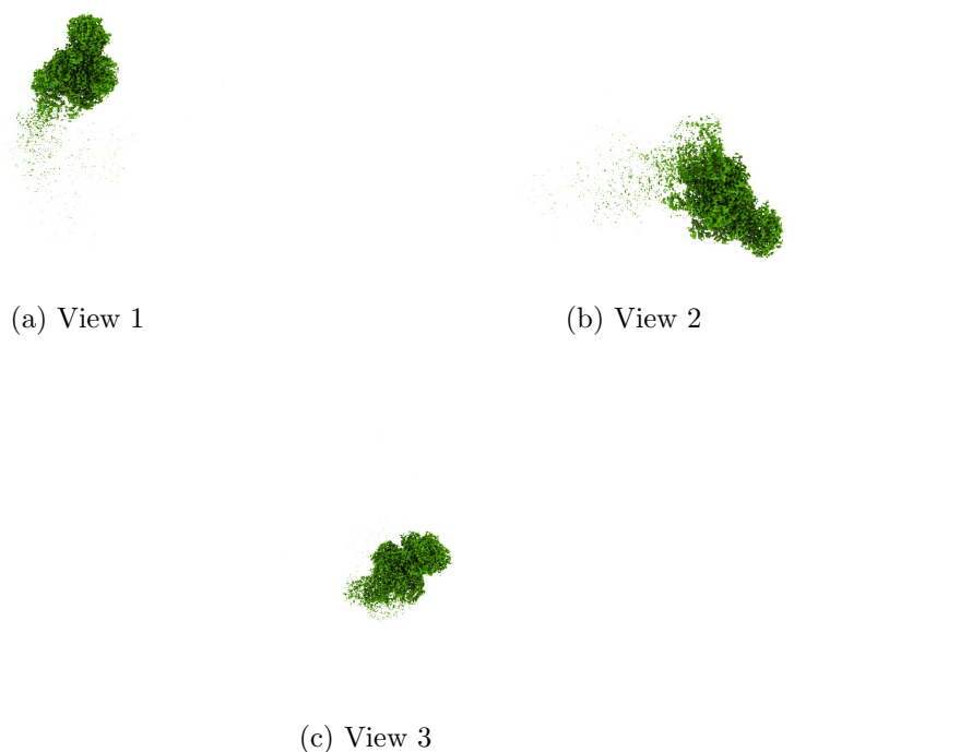
Figure 4: Isosurface at threshold=1.500000. Views generated by ChimeraX at a the following X, Y, Z angles: View 1 (0, -90, -90), View 2 (-90, 0, -90), View 3 (0, 0, 0).
