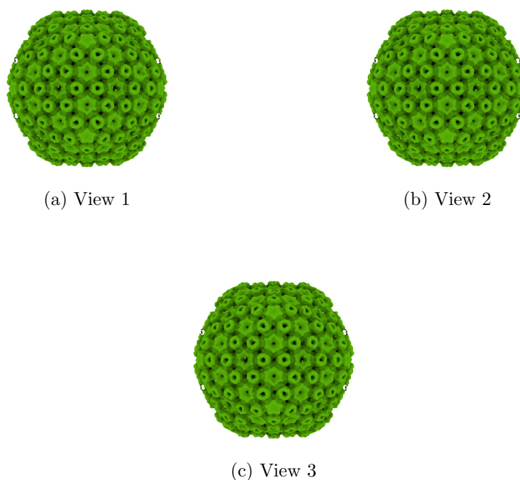
Figure 4: Isosurface at threshold=4150.000000. Views generated by ChimeraX at the following X, Y, Z angles: View 1 (0, -90, -90), View 2 (-90, 0, -90), View 3 (0, 0, 0).
