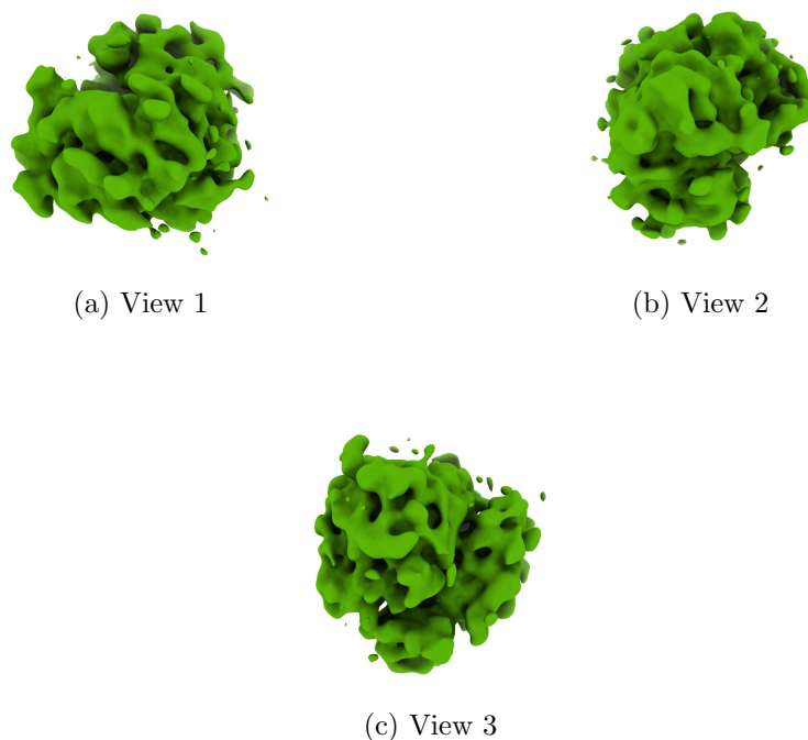
Figure 4: Isosurface at threshold=17.000000. Views generated by ChimeraX at a the following X, Y, Z angles: View 1 (0, -90, -90), View 2 (-90, 0, -90), View 3 (0, 0, 0).
