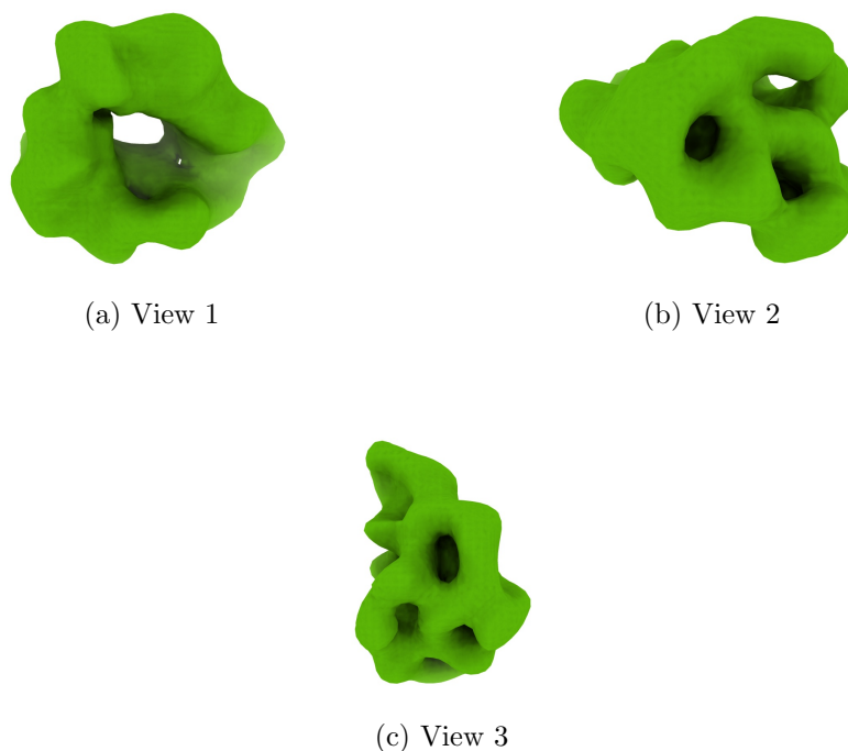
Figure 4: Isosurface at threshold=0.069000. Views generated by ChimeraX at a the following X, Y, Z angles: View 1 (0, -90, -90), View 2 (-90, 0, -90), View 3 (0, 0, 0).
