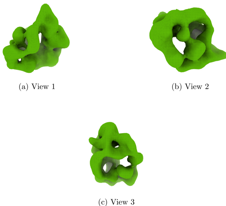
Figure 4: Isosurface at threshold=0.063000. Views generated by ChimeraX at a the following X, Y, Z angles: View 1 (0, -90, -90), View 2 (-90, 0, -90), View 3 (0, 0, 0).
