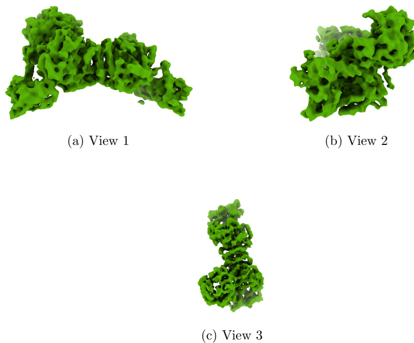
Figure 4: Isosurface at threshold=4.080000. Views generated by ChimeraX at a the following X, Y, Z angles: View 1 (0, -90, -90), View 2 (-90, 0, -90), View 3 (0, 0, 0).
