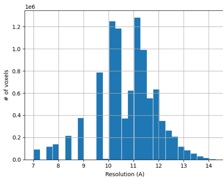
Figure 23: Histogram of the local resolution according to MonoRes.
