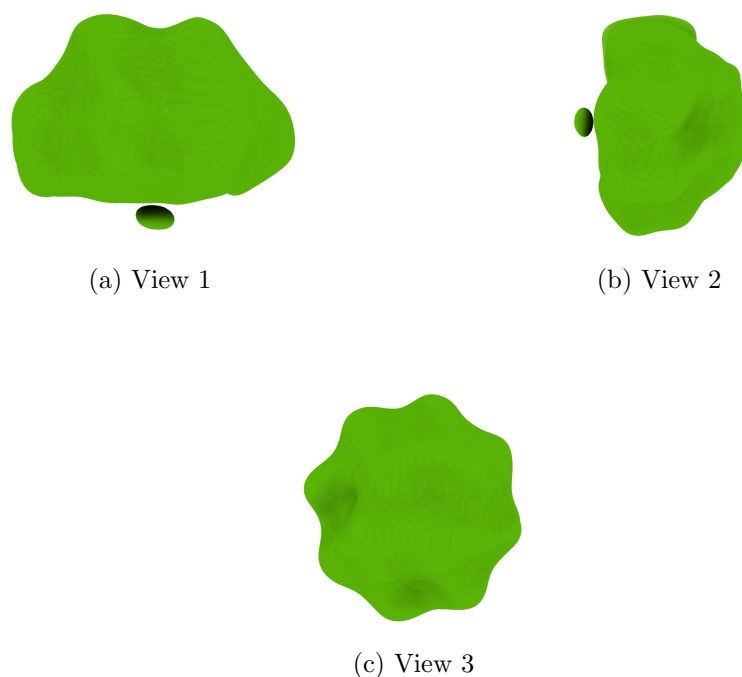
Figure 4: Isosurface at threshold=0.740000. Views generated by ChimeraX at a the following X, Y, Z angles: View 1 (0, -90, -90), View 2 (-90, 0, -90), View 3 (0, 0, 0).
