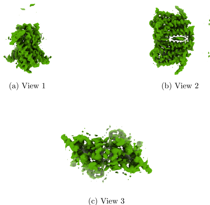
Figure 4: Isosurface at threshold=0.128000. Views generated by ChimeraX at a the following X, Y, Z angles: View 1 (0, -90, -90), View 2 (-90, 0, -90), View 3 (0, 0, 0).
