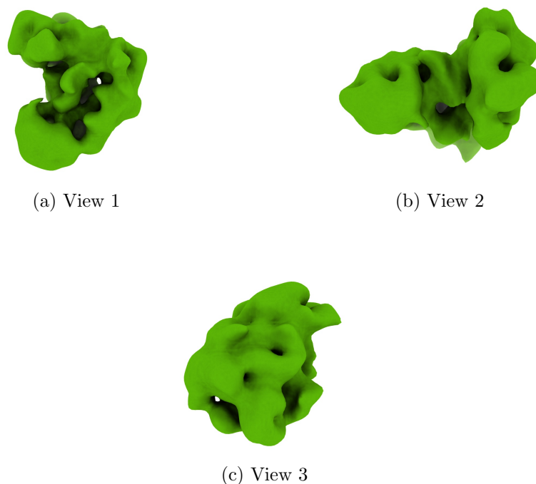
Figure 4: Isosurface at threshold=29.000000. Views generated by ChimeraX at a the following X, Y, Z angles: View 1 (0, -90, -90), View 2 (-90, 0, -90), View 3 (0, 0, 0).
