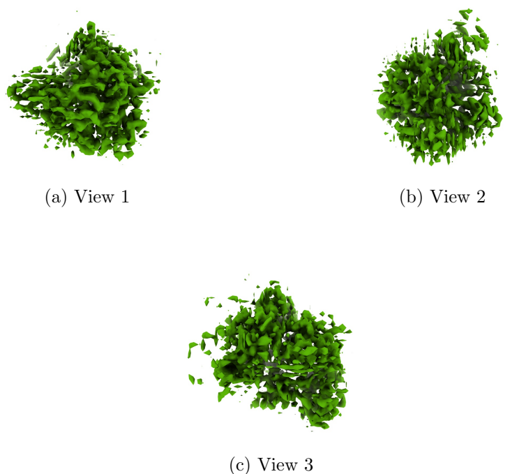
Figure 4: Isosurface at threshold=0.090000. Views generated by ChimeraX at a the following X, Y, Z angles: View 1 (0, -90, -90), View 2 (-90, 0, -90), View 3 (0, 0, 0).
