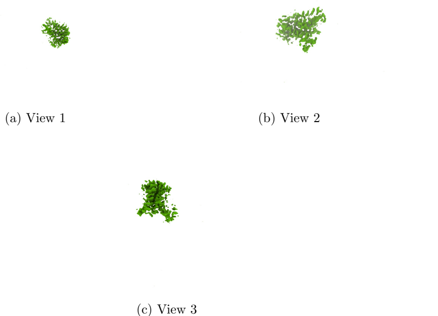
Figure 4: Isosurface at threshold=1.900000. Views generated by ChimeraX at a the following X, Y, Z angles: View 1 (0, -90, -90), View 2 (-90, 0, -90), View 3 (0, 0, 0).
