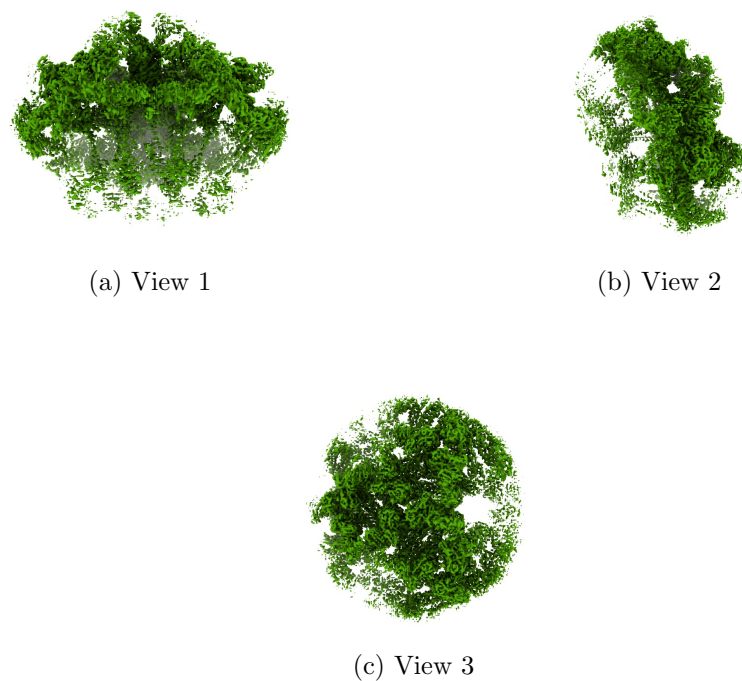
Figure 4: Isosurface at threshold=0.145000. Views generated by ChimeraX at a the following X, Y, Z angles: View 1 (0, -90, -90), View 2 (-90, 0, -90), View 3 (0, 0, 0).
