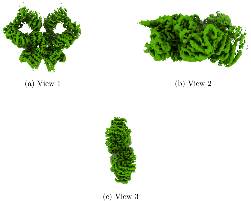
Figure 4: Isosurface at threshold=0.330000. Views generated by ChimeraX at a the following X, Y, Z angles: View 1 (0, -90, -90), View 2 (-90, 0, -90), View 3 (0, 0, 0).
