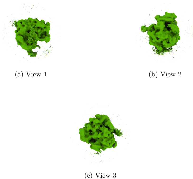
Figure 4: Isosurface at threshold=0.207000. Views generated by ChimeraX at a the following X, Y, Z angles: View 1 (0, -90, -90), View 2 (-90, 0, -90), View 3 (0, 0, 0).
