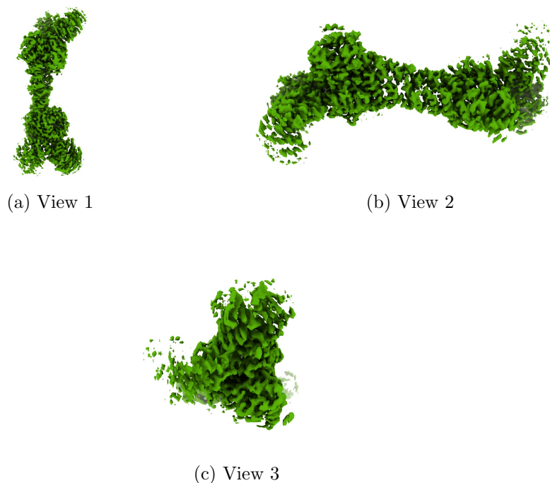
Figure 4: Isosurface at threshold=0.006280. Views generated by ChimeraX at a the following X, Y, Z angles: View 1 (0, -90, -90), View 2 (-90, 0, -90), View 3 (0, 0, 0).
