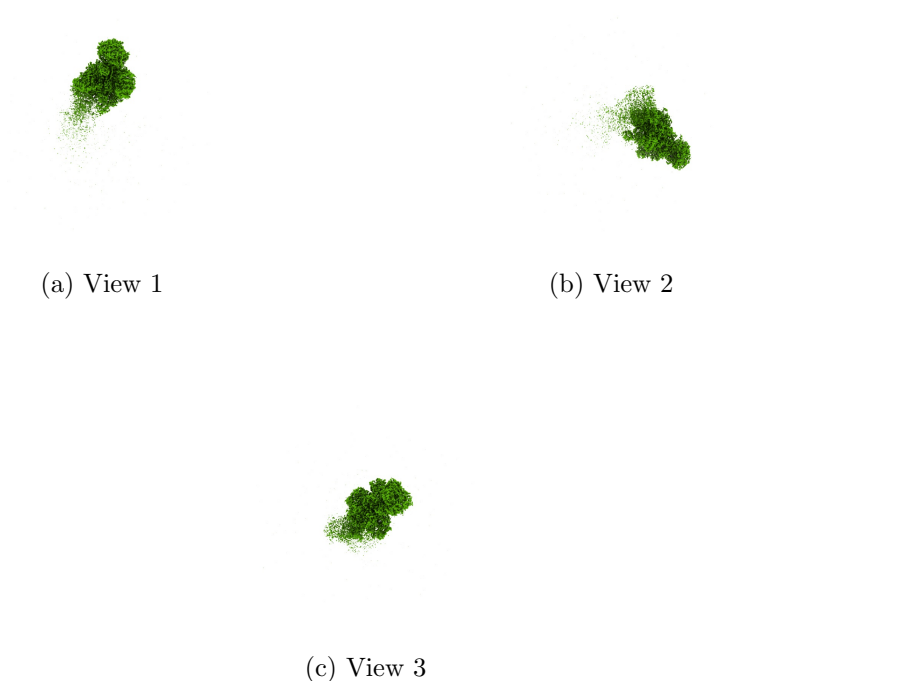
Figure 4: Isosurface at threshold=0.720000. Views generated by ChimeraX at a the following X, Y, Z angles: View 1 (0, -90, -90), View 2 (-90, 0, -90), View 3 (0, 0, 0).
