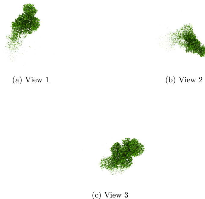
Figure 4: Isosurface at threshold=1.660000. Views generated by ChimeraX at a the following X, Y, Z angles: View 1 (0, -90, -90), View 2 (-90, 0, -90), View 3 (0, 0, 0).
