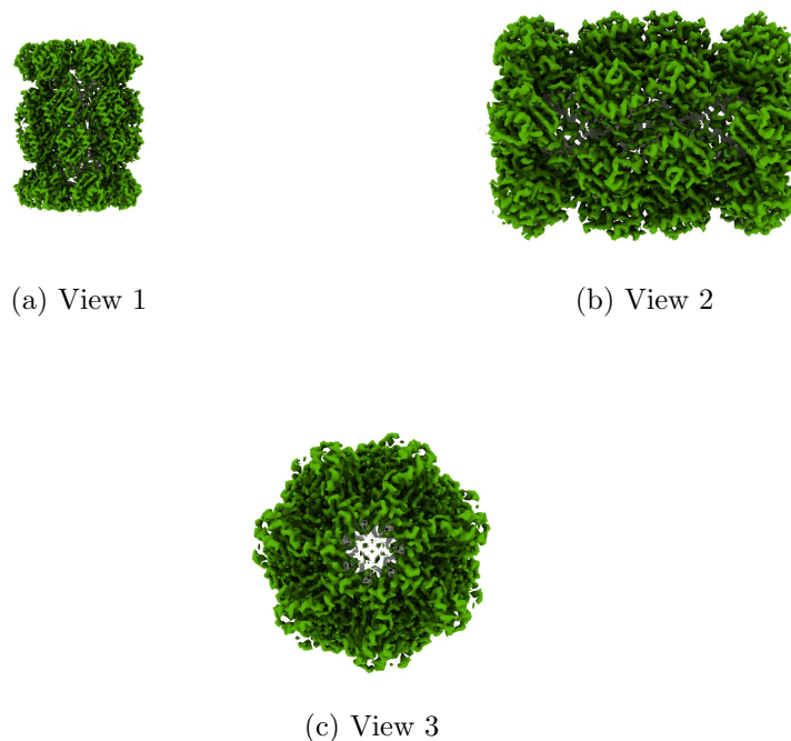
Figure 4: Isosurface at threshold=0.387000. Views generated by ChimeraX at a the following X, Y, Z angles: View 1 (0, -90, -90), View 2 (-90, 0, -90), View 3 (0, 0, 0).
