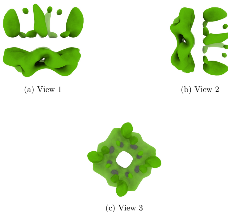
Figure 4: Isosurface at threshold=0.017700. Views generated by ChimeraX at a the following X, Y, Z angles: View 1 (0, -90, -90), View 2 (-90, 0, -90), View 3 (0, 0, 0).
