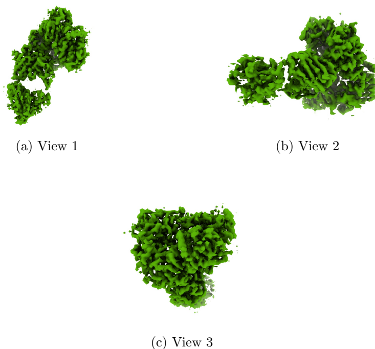
Figure 4: Isosurface at threshold=0.241000. Views generated by ChimeraX at a the following X, Y, Z angles: View 1 (0, -90, -90), View 2 (-90, 0, -90), View 3 (0, 0, 0).
