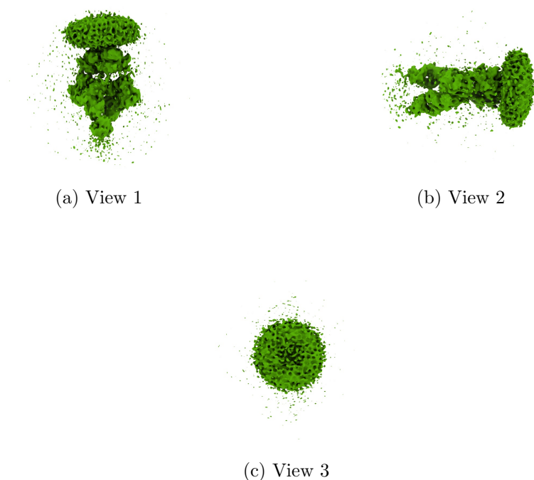
Figure 4: Isosurface at threshold=0.083000. Views generated by ChimeraX at a the following X, Y, Z angles: View 1 (0, -90, -90), View 2 (-90, 0, -90), View 3 (0, 0, 0).
