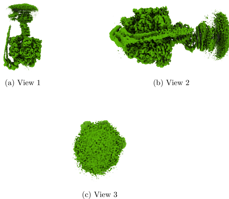
Figure 4: Isosurface at threshold=0.036500. Views generated by ChimeraX at a the following X, Y, Z angles: View 1 (0, -90, -90), View 2 (-90, 0, -90), View 3 (0, 0, 0).
