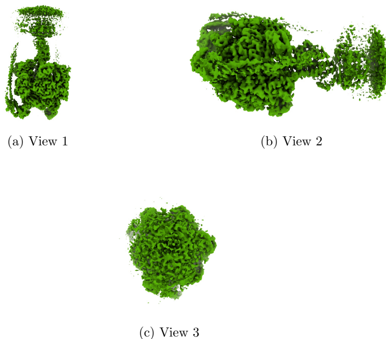
Figure 4: Isosurface at threshold=0.043200. Views generated by ChimeraX at a the following X, Y, Z angles: View 1 (0, -90, -90), View 2 (-90, 0, -90), View 3 (0, 0, 0).
