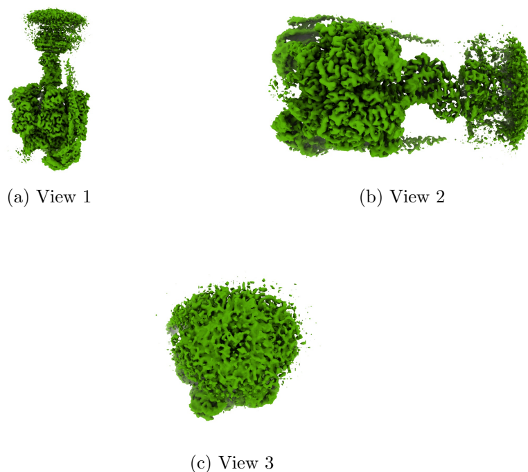
Figure 4: Isosurface at threshold=0.039600. Views generated by ChimeraX at a the following X, Y, Z angles: View 1 (0, -90, -90), View 2 (-90, 0, -90), View 3 (0, 0, 0).
