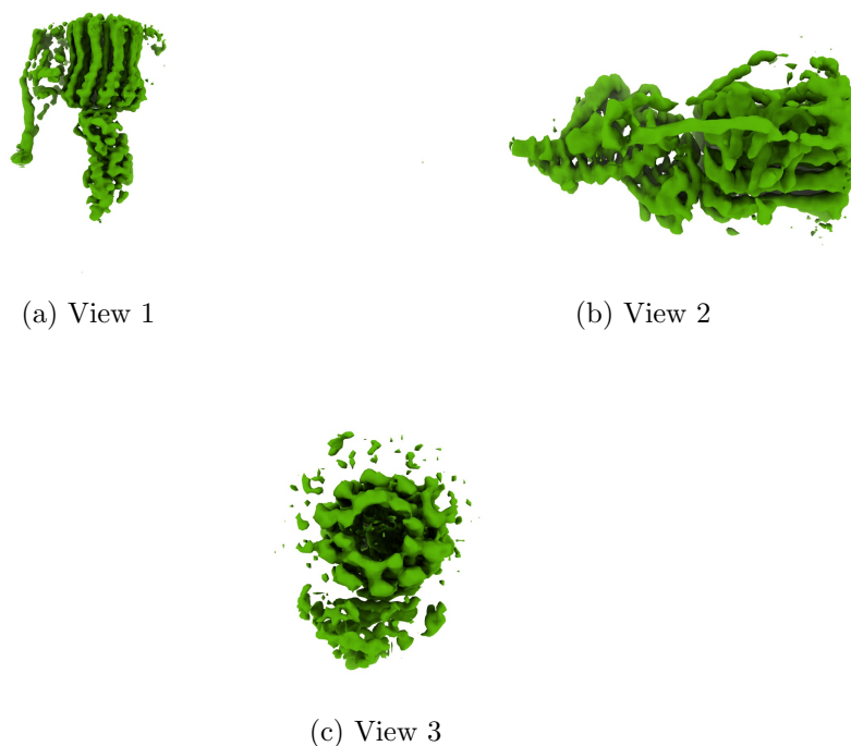
Figure 4: Isosurface at threshold=0.051500. Views generated by ChimeraX at a the following X, Y, Z angles: View 1 (0, -90, -90), View 2 (-90, 0, -90), View 3 (0, 0, 0).
