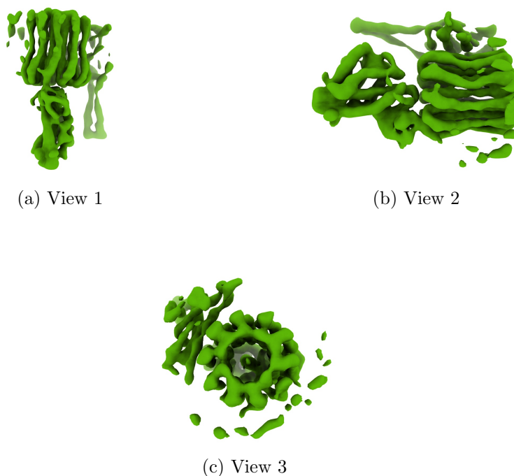
Figure 4: Isosurface at threshold=0.049100. Views generated by ChimeraX at a the following X, Y, Z angles: View 1 (0, -90, -90), View 2 (-90, 0, -90), View 3 (0, 0, 0).
