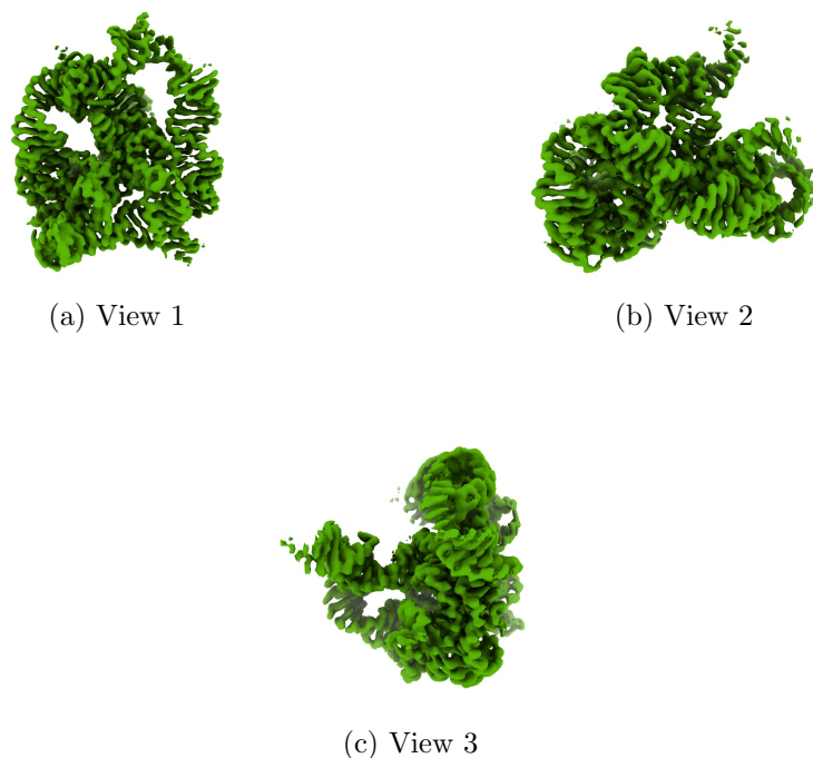
Figure 4: Isosurface at threshold=0.074000. Views generated by ChimeraX at a the following X, Y, Z angles: View 1 (0, -90, -90), View 2 (-90, 0, -90), View 3 (0, 0, 0).
