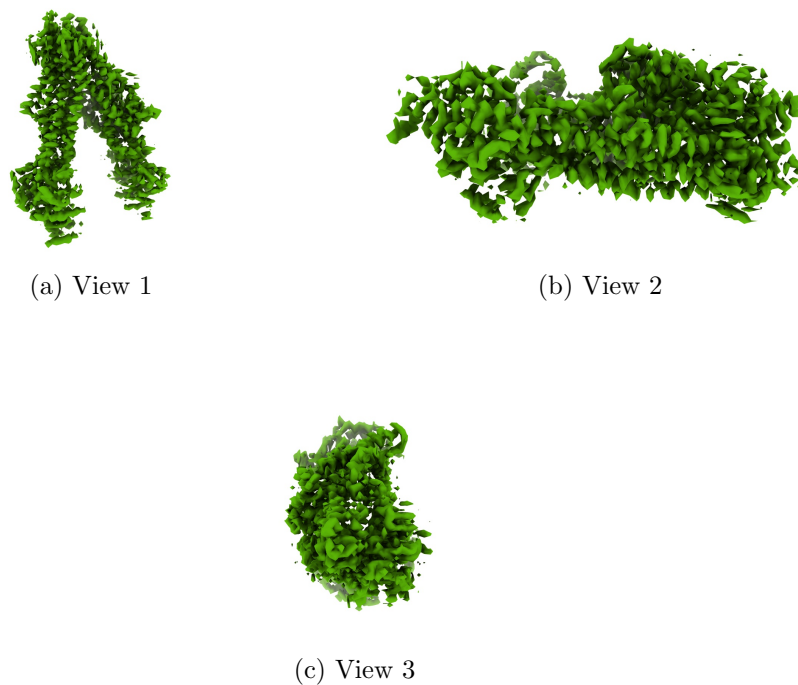
Figure 4: Isosurface at threshold=0.057200. Views generated by ChimeraX at a the following X, Y, Z angles: View 1 (0, -90, -90), View 2 (-90, 0, -90), View 3 (0, 0, 0).
