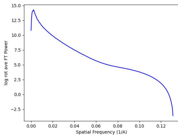
Figure 28: Logarithm of the radial average of the input map power in Fourier space.
