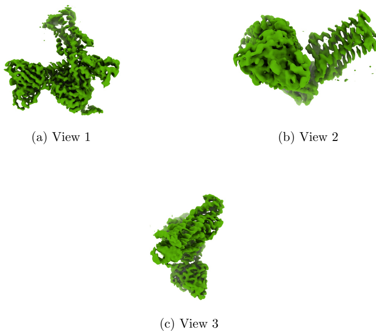
Figure 4: Isosurface at threshold=0.522000. Views generated by ChimeraX at a the following X, Y, Z angles: View 1 (0, -90, -90), View 2 (-90, 0, -90), View 3 (0, 0, 0).
