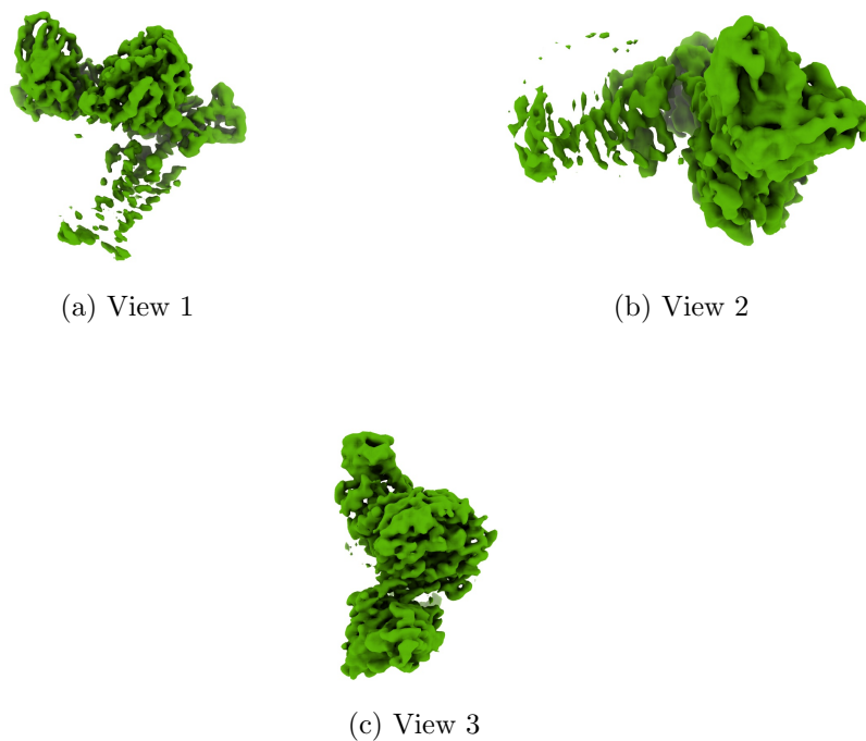
Figure 4: Isosurface at threshold=0.045600. Views generated by ChimeraX at a the following X, Y, Z angles: View 1 (0, -90, -90), View 2 (-90, 0, -90), View 3 (0, 0, 0).
