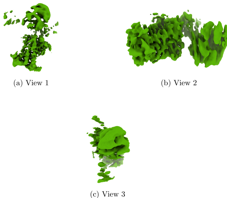
Figure 4: Isosurface at threshold=0.039800. Views generated by ChimeraX at a the following X, Y, Z angles: View 1 (0, -90, -90), View 2 (-90, 0, -90), View 3 (0, 0, 0).
