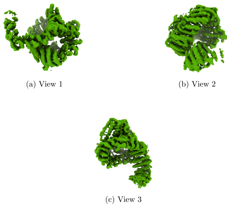
Figure 4: Isosurface at threshold=0.009650. Views generated by ChimeraX at a the following X, Y, Z angles: View 1 (0, -90, -90), View 2 (-90, 0, -90), View 3 (0, 0, 0).
