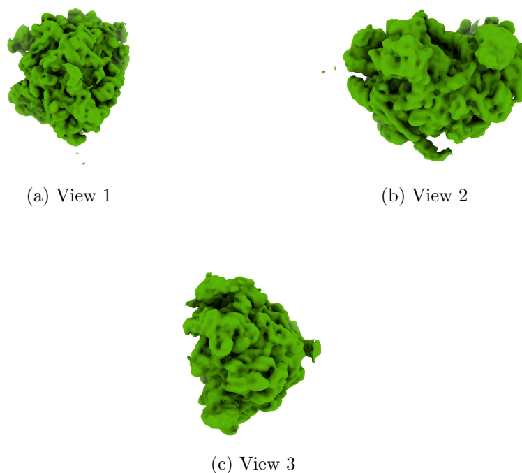
Figure 4: Isosurface at threshold=0.017000. Views generated by ChimeraX at the following X, Y, Z angles: View 1 (0, -90, -90), View 2 (-90, 0, -90), View 3 (0, 0, 0).
