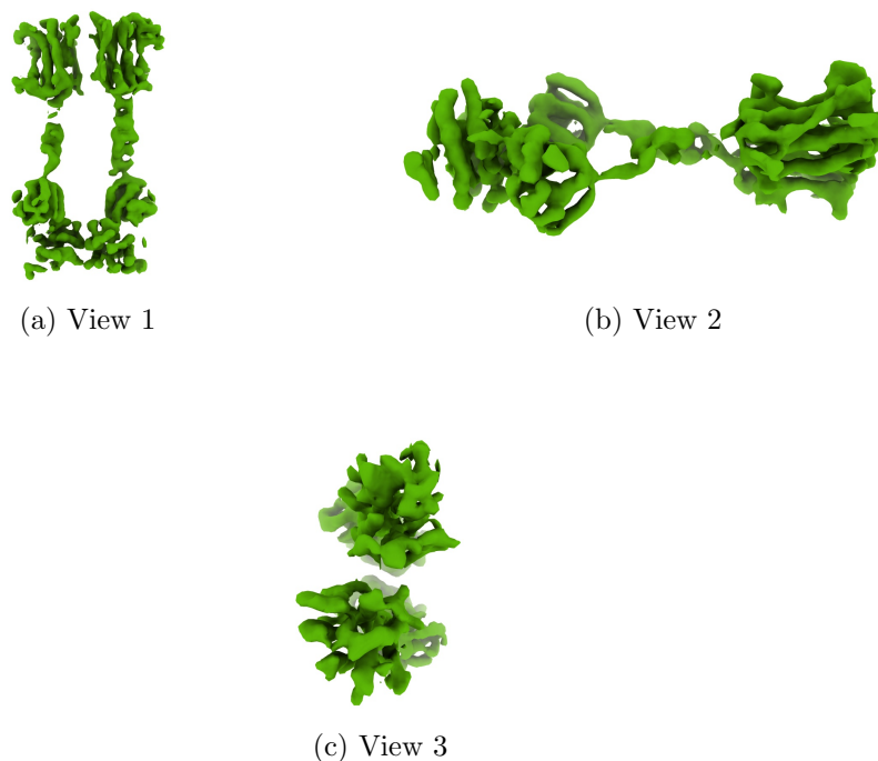
Figure 4: Isosurface at threshold=0.297000. Views generated by ChimeraX at a the following X, Y, Z angles: View 1 (0, -90, -90), View 2 (-90, 0, -90), View 3 (0, 0, 0).
