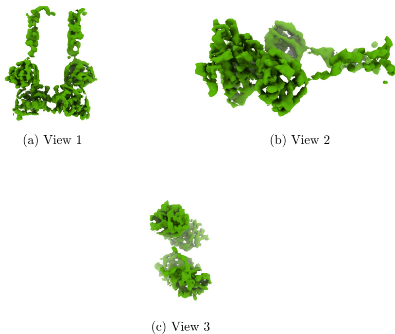
Figure 4: Isosurface at threshold=0.353000. Views generated by ChimeraX at a the following X, Y, Z angles: View 1 (0, -90, -90), View 2 (-90, 0, -90), View 3 (0, 0, 0).
