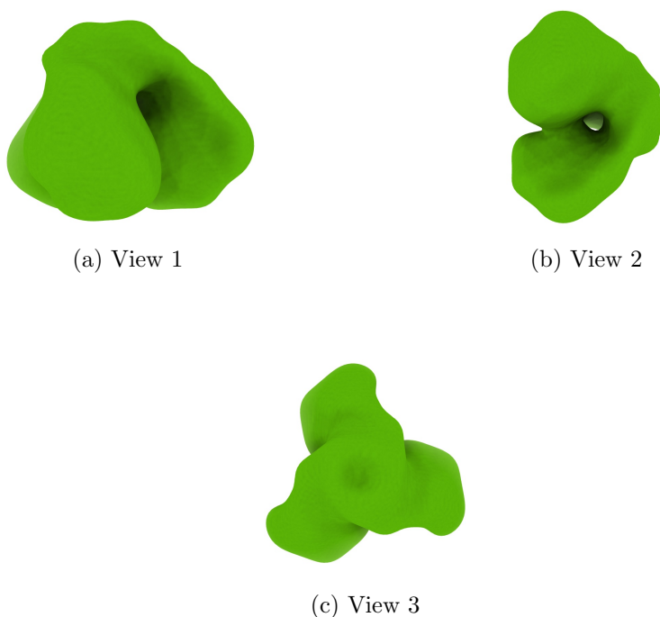
Figure 4: Isosurface at threshold=4.170000. Views generated by ChimeraX at a the following X, Y, Z angles: View 1 (0, -90, -90), View 2 (-90, 0, -90), View 3 (0, 0, 0).
