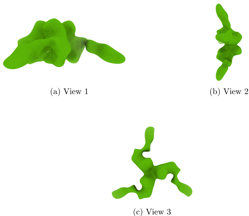
Figure 4: Isosurface at threshold=34.400000. Views generated by ChimeraX at a the following X, Y, Z angles: View 1 (0, -90, -90), View 2 (-90, 0, -90), View 3 (0, 0, 0).
