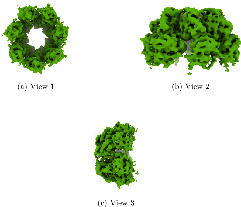
Figure 4: Isosurface at threshold=0.150000. Views generated by ChimeraX at the following X, Y, Z angles: View 1 (0, -90, -90), View 2 (-90, 0, -90), View 3 (0, 0, 0).
