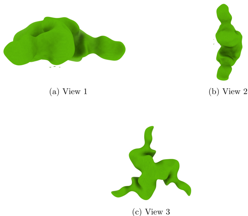
Figure 4: Isosurface at threshold=1.740000. Views generated by ChimeraX at a the following X, Y, Z angles: View 1 (0, -90, -90), View 2 (-90, 0, -90), View 3 (0, 0, 0).
